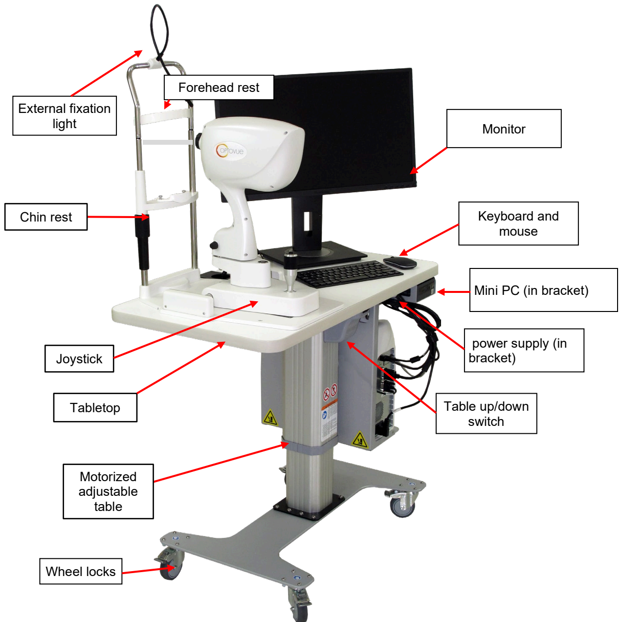
Figure 1 Current iVue with mini PC
