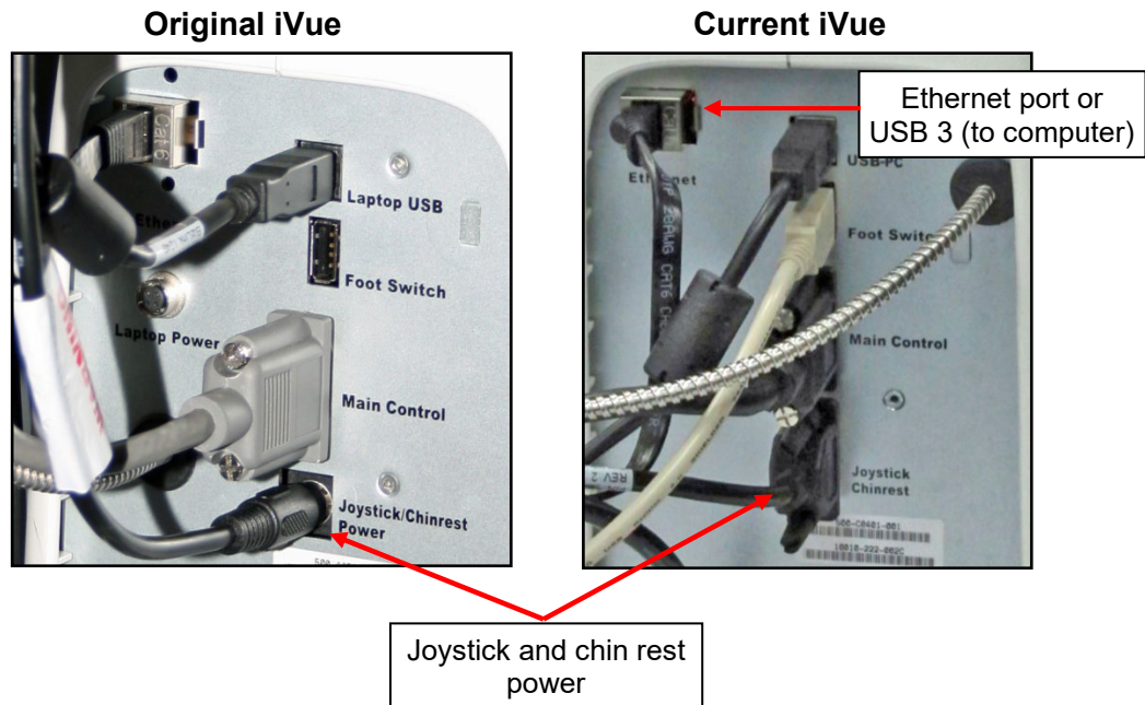
Figure 3 Original vs. Current Connection
