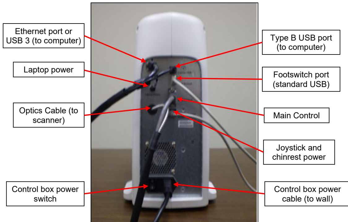
Figure 2 Control Box Cable Connections (Current)
